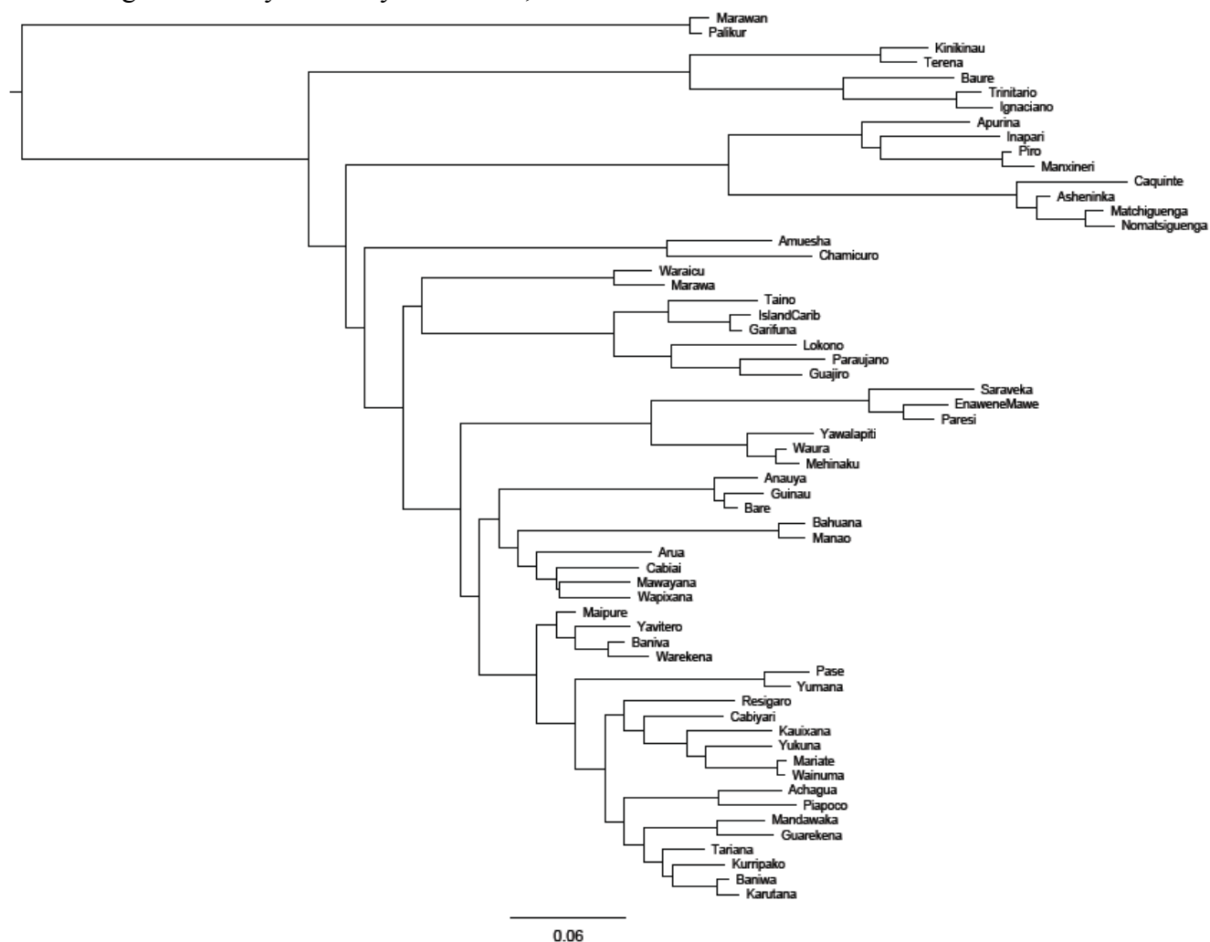
Figure S2. Phylogram equivalent of Figure 2. Maximum clade credibility tree from 1,000 Bayesian Markov chain Monte Carlo trees.
